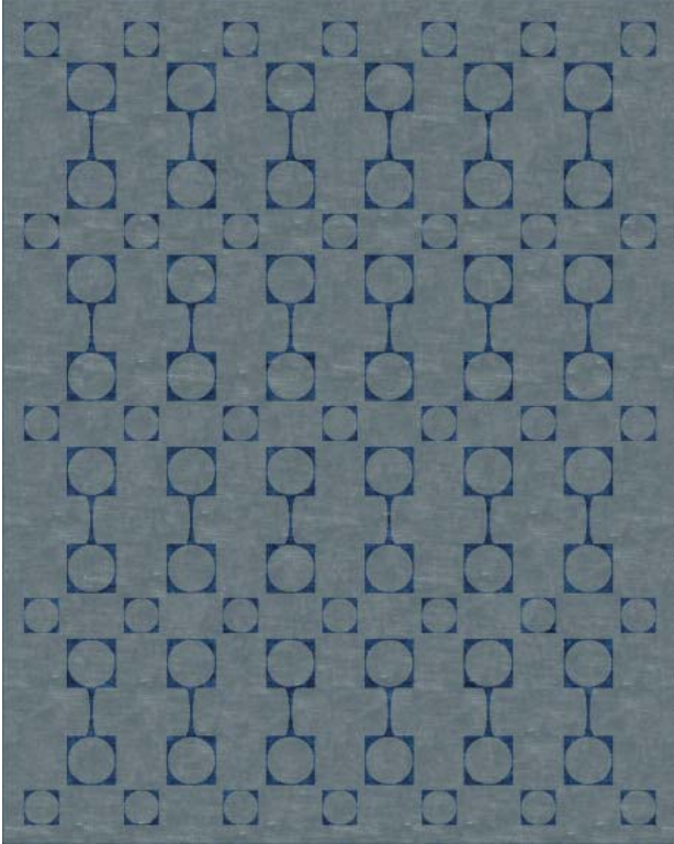
EQUATION - OCEAN
